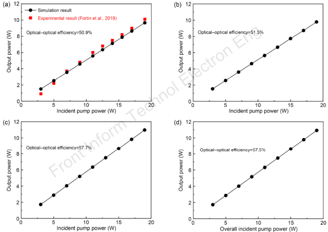
Fig. 2 Comparison of the simulation results and experimental results from Fortin et al. (2019) (a) and simulated output power of the \text{Dy}^{3+} -doped fluoride fiber laser as a function of the incident pump power with different pumping methods: forward pumping (b), backward pumping (c), and bi-directional pumping (d)
