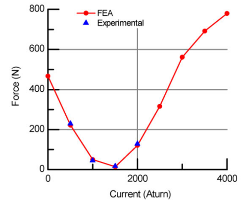
Fig. 12 Inverse current excitation effects on the F_H of MHVA
