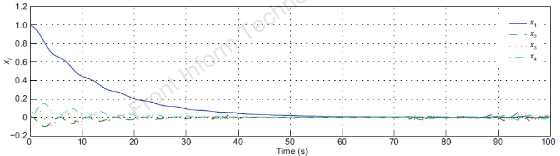
Fig. 4 Trajectories of system states with random cryptographic protection of probability \bar{\alpha} = 0.279 under random zero-measurement attacks of probability \bar{\beta} = 1
