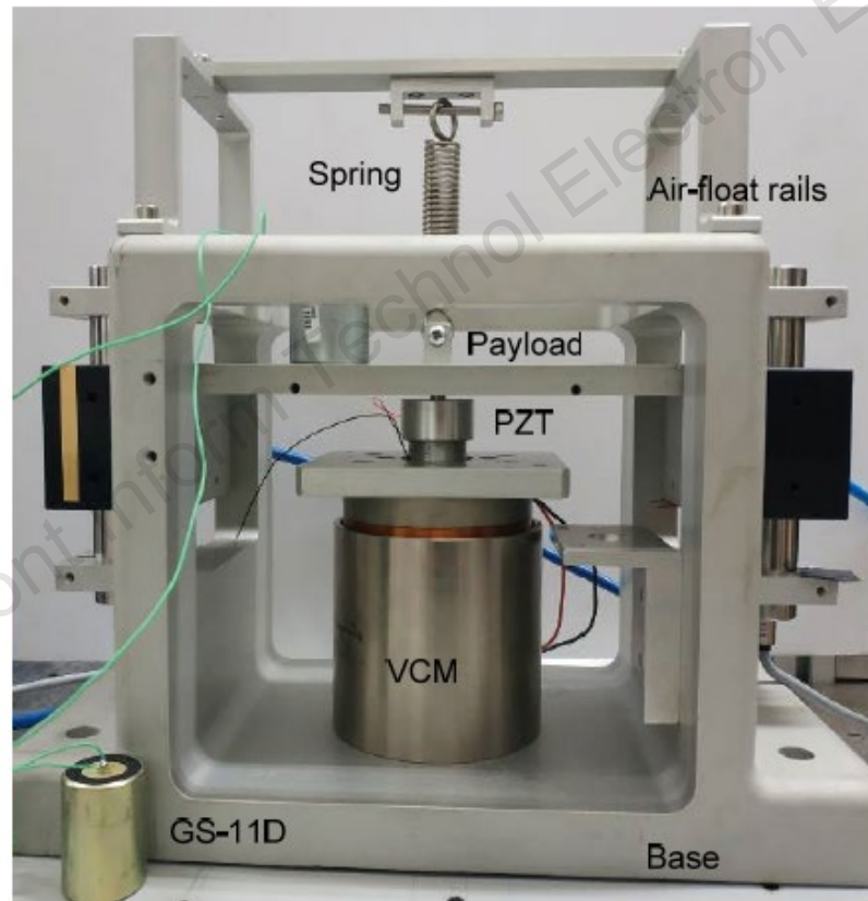
Fig. 9 Physical picture of the designed DSA-SAVIS
