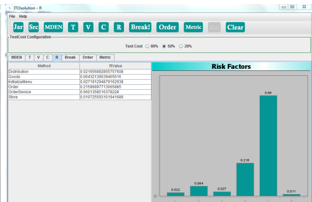
(b) The risk distribution diagram of the example code
