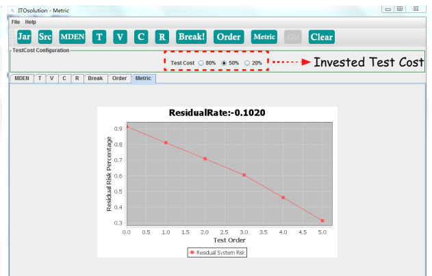
(d) The software risk reduction curve due to the integration steps
