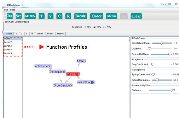
(a) The MDEN model mapped from the example code
