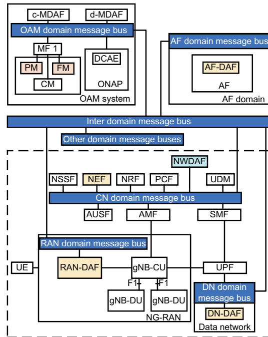
Fig. 6 Enhanced integrated data analysis framework (Pateromichelakis et al., 2019)
