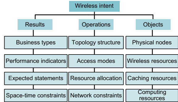
Fig. 8 Wireless intent language model
