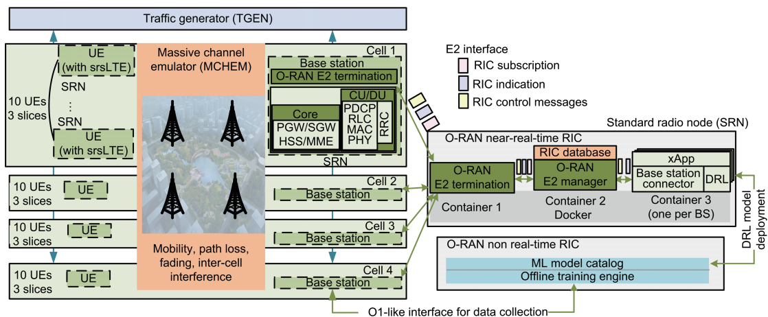
Fig. 10 O-RAN integration in Colosseum (Bonati et al., 2020)
