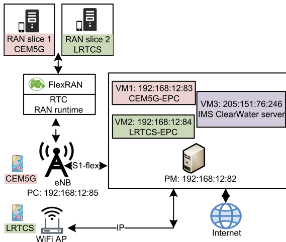
Fig. 9 System structure of the experimental scenario (Issa et al., 2019)
