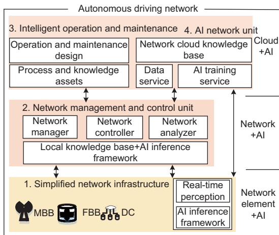
Fig. 1 Solution to the autonomous driving network (Huawei, 2020)
