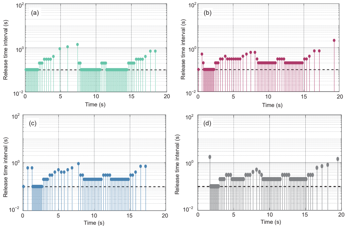
Fig. 3 Transmission instants and release time intervals in the simulations: (a) 1 st vehicle; (b) 2 nd vehicle; (c) 3 rd vehicle; (d) 4 th vehicle
