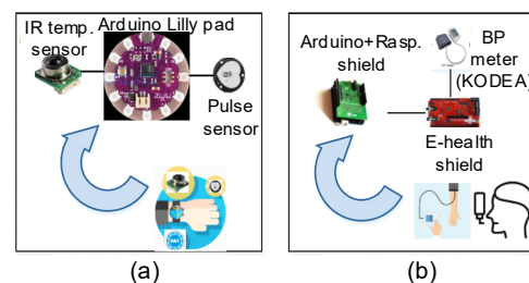
Fig. 25 Setup of wearable (a) and non-wearable (b) devices Reprinted from Ashraf et al. (2020), Copyright 2020, with permission from IEEE
