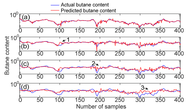
Fig. 11 Prediction results in the debutanizer column: (a) LWSBN; (b) LWBN; (c) LWSLFA; (d) LWLR References to color refer to the online version of this figure
