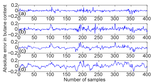
Fig. 13 Prediction of absolute errors in the debutanizer column: (a) LWSBN; (b) LWBN; (c) LWSLFA; (d) LWLR
