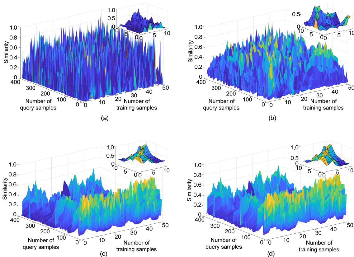
Fig. 12 Similarity diagrams in the debutanizer column: (a) LWSBN; (b) LWBN; (c) LWSLFA; (d) LWLR References to color refer to the online version of this figure
