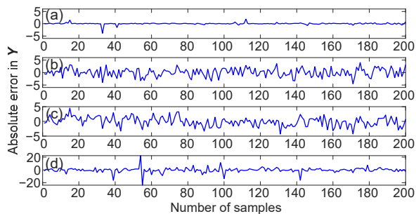
Fig. 10 Prediction of absolute errors in a numerical example: (a) LWSBN; (b) LWBN; (c) LWSLFA; (d) LWLR
