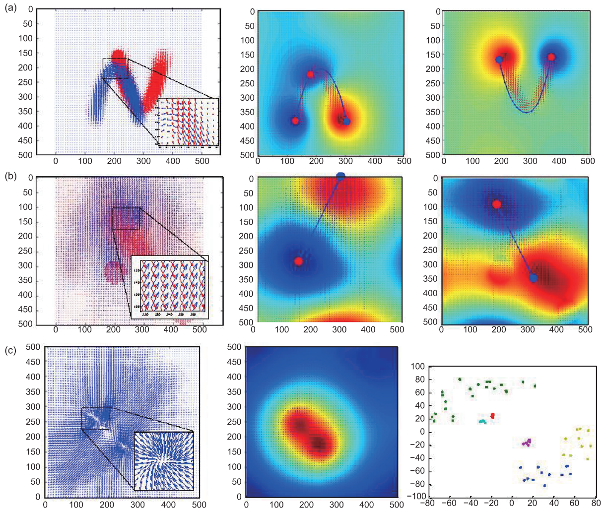
Fig. 14 Results of the synthetic motion pattern dataset: (a) MFF and the two trajectories of the double-V crossing motion pattern; (b) MFF and the two trajectories of the crossing motion pattern; (c) MFF and the trajectories of the gathering motion pattern
