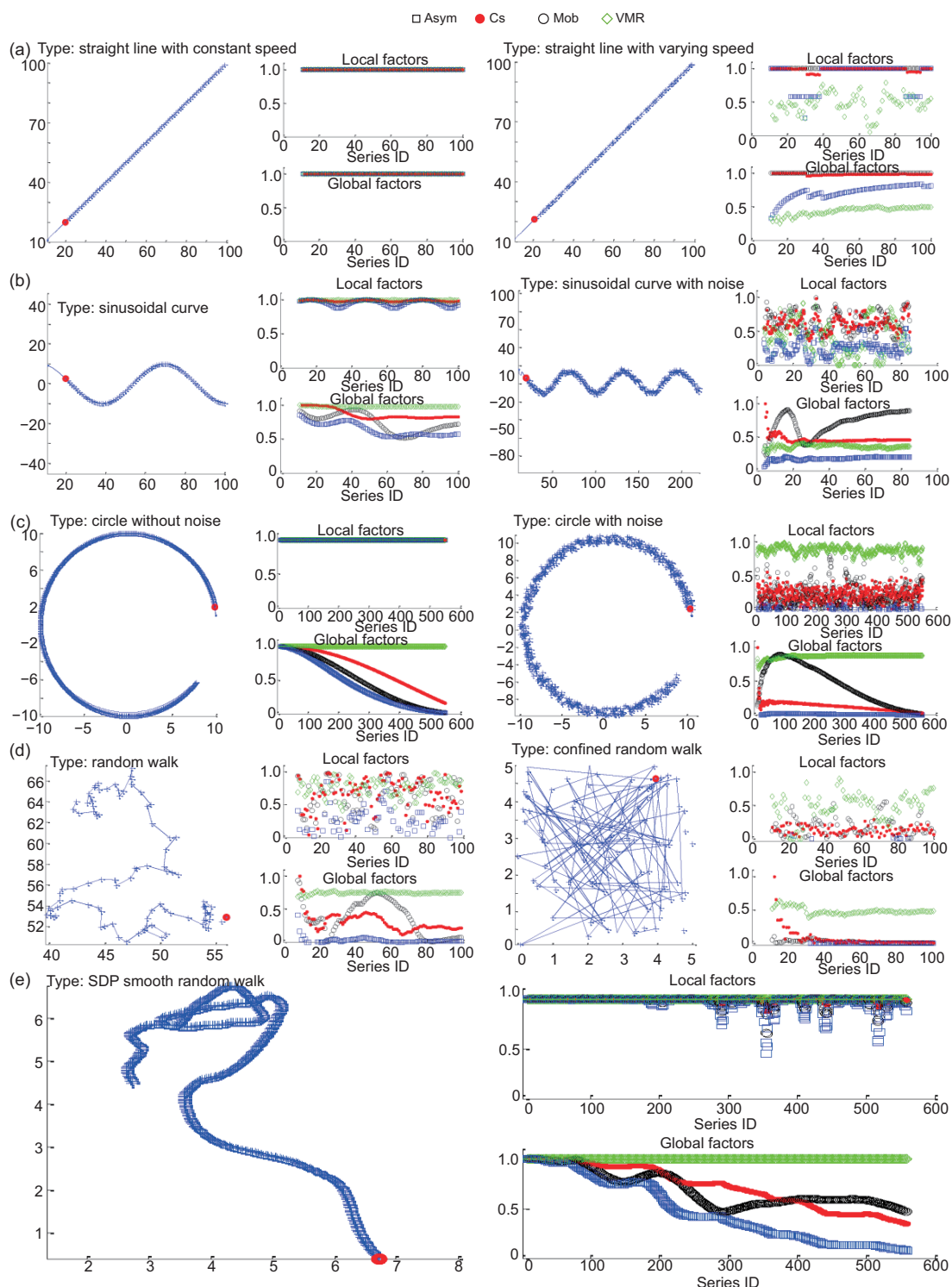
Fig. 3 Purposiveness evaluation of the synthetic dataset: (a) a line trajectory with a stable speed (left) and a line trajectory with an unstable speed (right); (b) a sinusoidal curve (left) and a sinusoidal curve trajectory with heavy noise (right); (c) a smooth circle trajectory (left) and a smooth circle trajectory with noise (right); (d) a Brownian random walk trajectory (left) and a confined random walk trajectory (right); (e) a self-driven particle's trajectory
