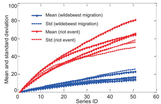
Fig. 18 Comparison of two typical crowd motions. References to color refer to the online version of this figure
