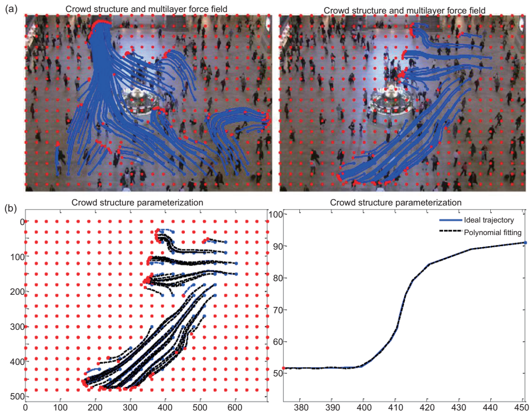
Fig. 10 Ideal trajectory parameterization of the grand central station: (a) unified ideal trajectories for the representation of crowd structure; (b) ideal trajectory parameterization
