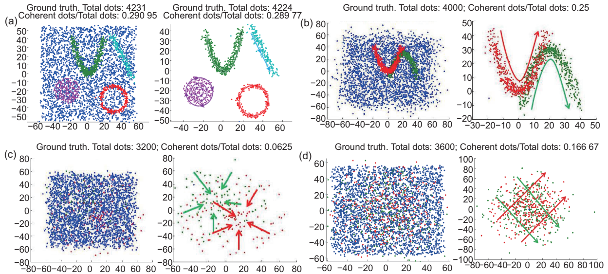
Fig. 11 Synthetic datasets: (a) there are four motion patterns generated by the parabola, circle, line, and disk with heavy noise (left) and without noise (right); (b) there are two groups of particles with double-V patterns with high levels of noise (left) and without noise (right); (c) there are two groups of sparse particles with high levels of noise (left) and without noise (right); (d) two hundred sparse particles gather toward two destination regions with high levels of noise (left) and without noise (right)
