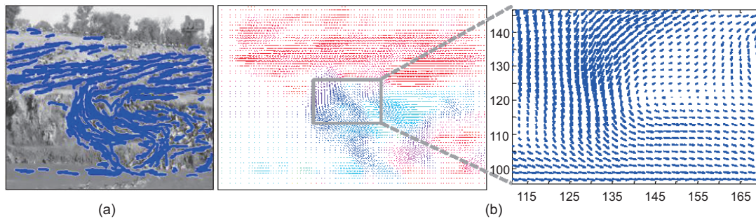
Fig. 6 MFF of the wildebeest migration video: (a) a motion field made by optical flow; (b) MFF x_{img} and y_{img} denote the horizontal and vertical axes of the image plane in the unit of pixel, respectively. In (b), red means the direction of the velocity vector is ranged in 0^\circ - 60^\circ , and blue is 120^\circ - 180^\circ . References to color refer to the online version of this figure
