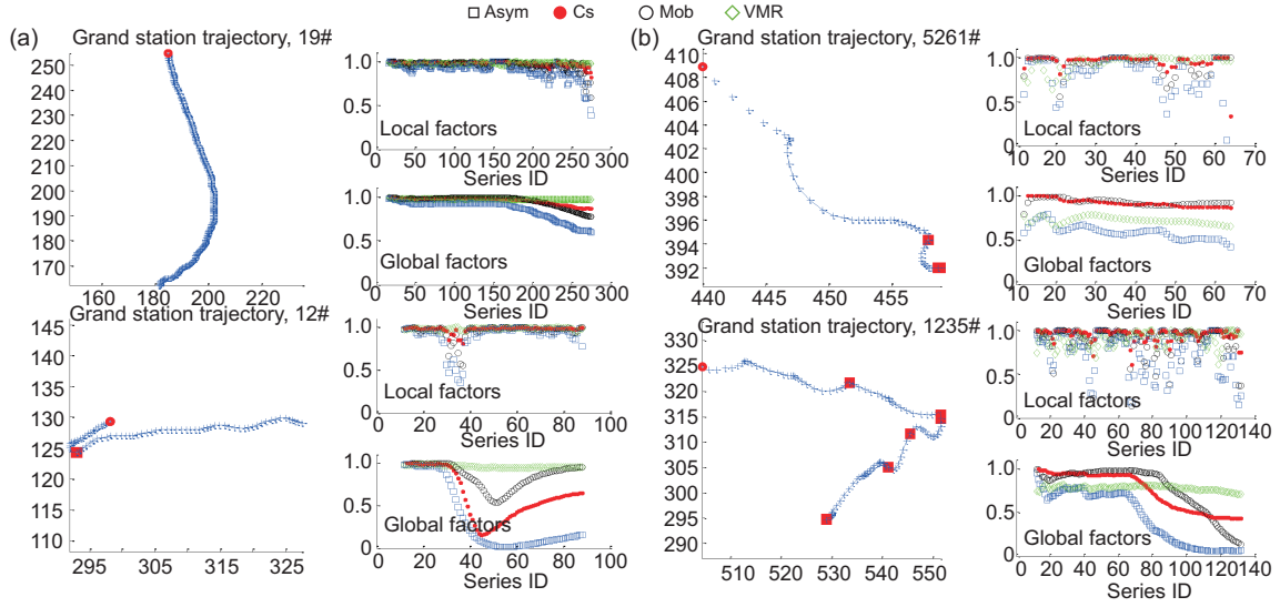
Fig. 4 Purposiveness evaluation of the real dataset: (a) the 19 th trajectory (upper) and the 12 th trajectory (lower); (b) the 5261 st trajectory (upper) and the 1235 th trajectory (lower)
