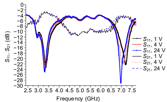
Fig. 4 Experimental results of S_{11} and S_{21} spectra of the SIR when the applied voltage is 1, 4, or 24 V
