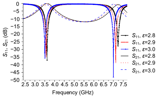
Fig. 3 Simulation results of S_{11} and S_{21} spectra of the SIR when the liquid crystal dielectric constant varies from 2.8 to 3.0
