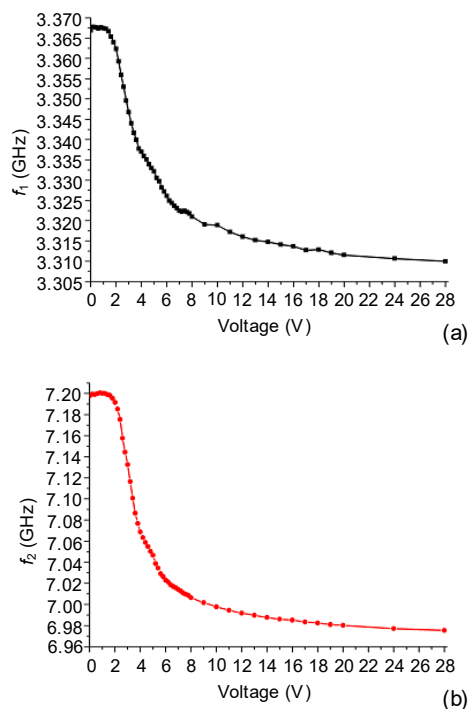
Fig. 5 Experimental results of the resonant frequency as a function of the applied voltage: (a) low resonant frequency f_1 ; (b) high resonant frequency f_2
