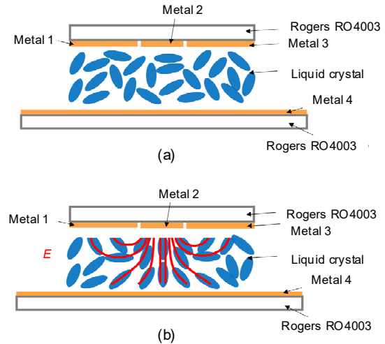
Fig. 2 Liquid crystal molecule distribution of the SIR: (a) voltage off state ( V=0 ); (b) voltage on state ( V>0 )
