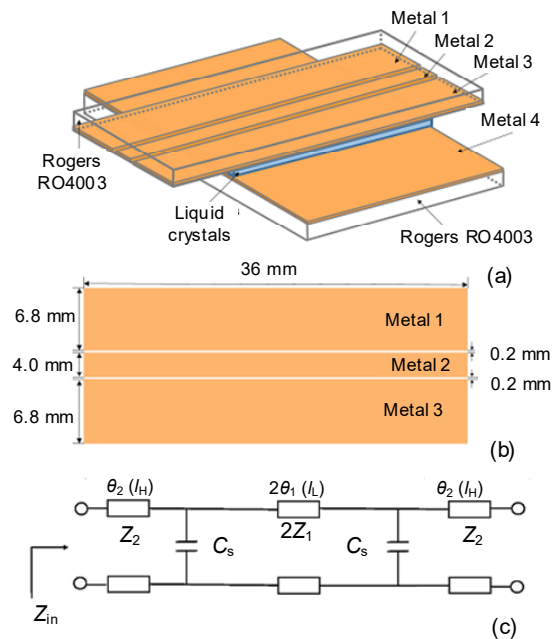
Fig. 1 Schematic of the proposed liquid-crystal-based CPW SIR (a), structure of the transmission line (b), and configuration of the SIR (c)
