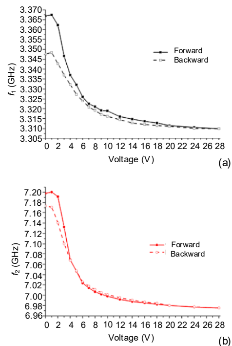
Fig. 6 Measured hysteresis loops of the resonant frequency under different electric fields: (a) low resonant frequency f_1 ; (b) high resonant frequency f_2
