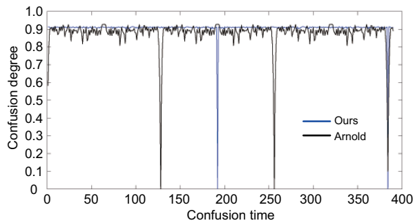
Fig. 7 Comparison of the gray value confusion degree with double cycles
