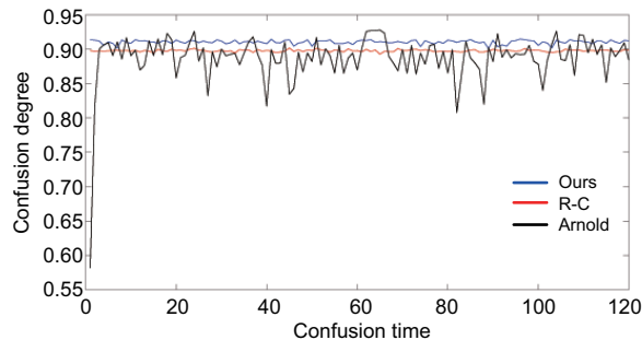
Fig. 8 Comparison of the gray value confusion degree with three methods in one cycle
