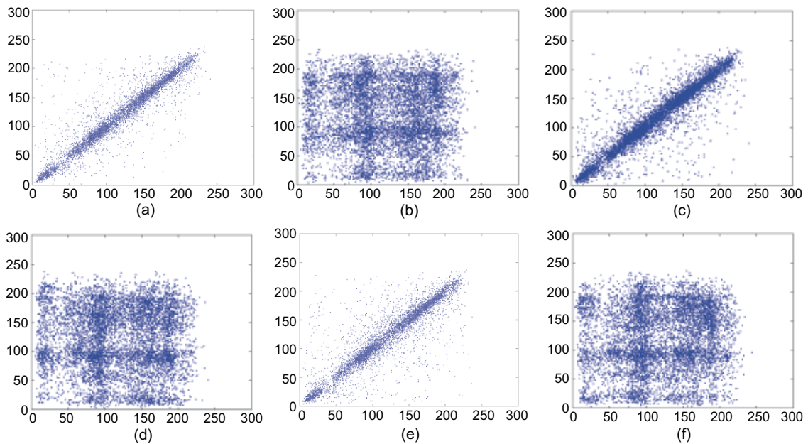
Fig. 4 Correlation of adjacent pixels in the Peppers image: (a) original image in the horizontal direction; (b) confused image in the horizontal direction; (c) original image in the vertical direction; (d) confused image in the vertical direction; (e) original image in the diagonal direction; (f) confused image in the diagonal direction
