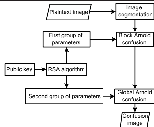
Fig. 2 Asymmetric image confusion algorithm
