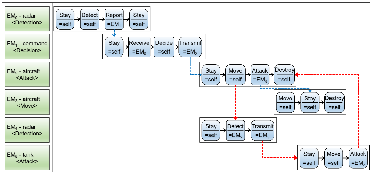
Fig. 11 Process-based modeling showing the radar's function of detecting the aircraft with the stealth function
