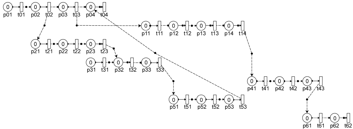
Fig. 12 A process-based Petri-net model showing aircraft with a stealth function
