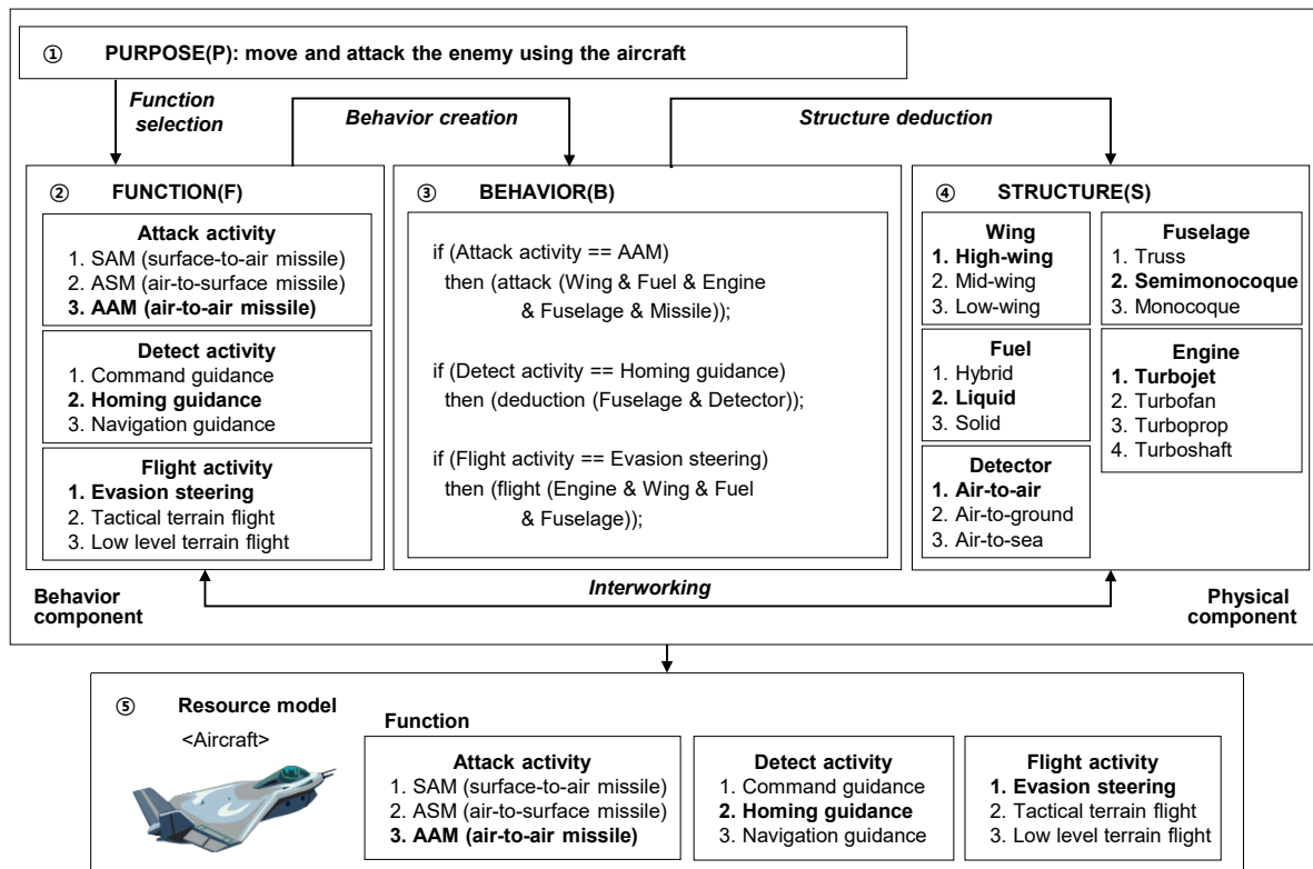
Fig. 3 An aircraft creation example based on the function–behavior–structure method
