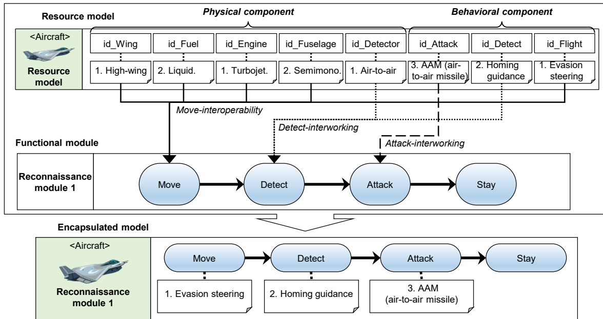
Fig. 6 An example of an encapsulated model combining a resource model and a functional module
