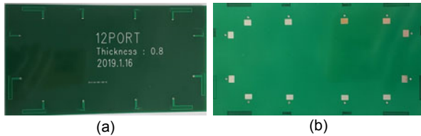
Fig. 10 Dual-module MIMO antenna: (a) top view of the antenna; (b) back view of the antenna
