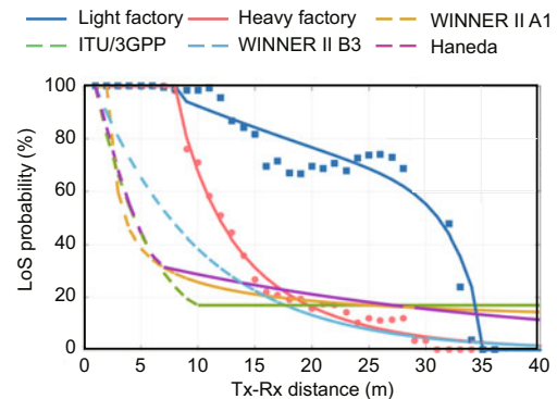
Fig. 12 LoS probability for light and heavy industry
