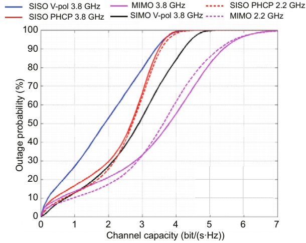
Fig. 13 SISO, SIMO, and MIMO channel capacities (SNR=10 dB)
