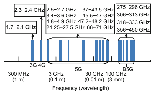
Fig. 9 Bands used for mobile communications
