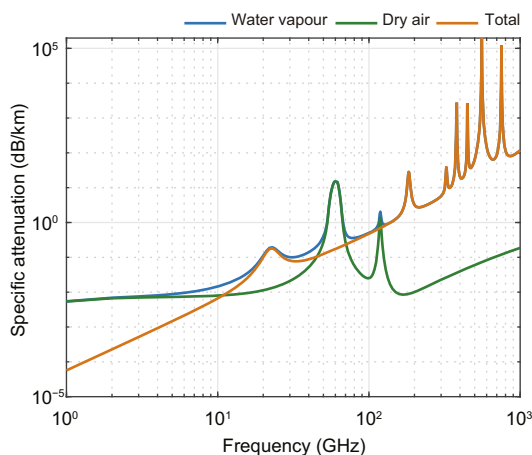
Fig. 6 Specific attenuation due to atmospheric gases (ITU-R, 2013)
