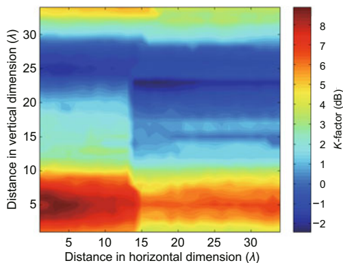
Fig. 7 K-factor values observed across the antenna array
