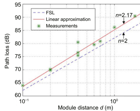
Fig. 10 Indoor path loss averaged between 300 and 310 GHz
