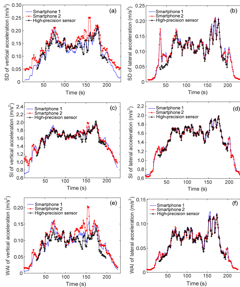
Fig. 12 Comparison of evaluation indexes with 5-s moving window: SD (a), SI (c), and WAI (e) of the vertical acceleration, and SD (b), SI (d), and WAI (f) of the lateral acceleration
