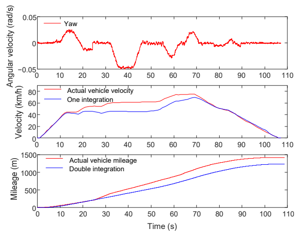
Fig. 16 Vehicle yaw angular velocity, speed, and location
