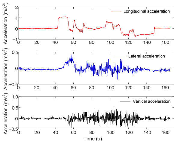
Fig. 15 Vehicle vibration acceleration
