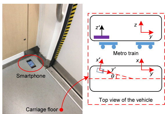
Fig. 7 Placement points of the smartphone during the field test
