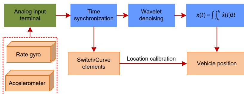
Fig. 5 Flowchart of vehicle location correction
