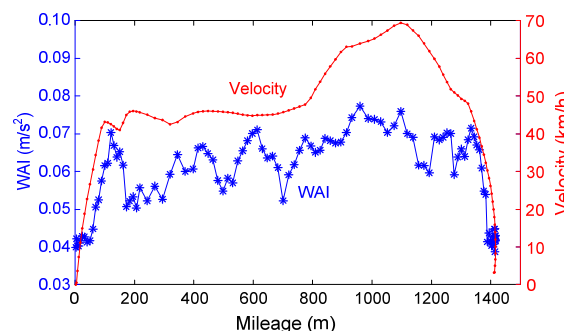
Fig. 19 Vehicle ride comfort WAI and velocity in relation to mileage (References to color refer to the online version of this figure)
