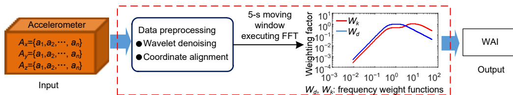
Fig. 6 Process of calculating the weighted acceleration index (WAI)
