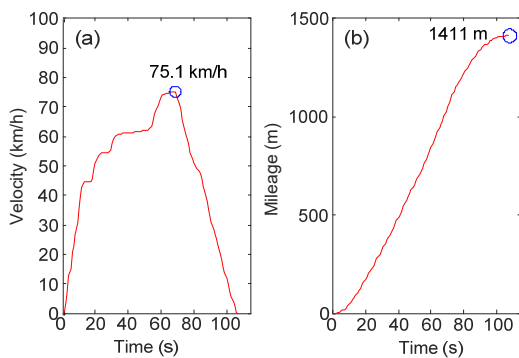
Fig. 13 Actual vehicle velocity (a) and mileage (b)
