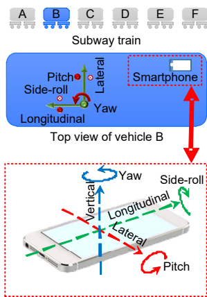
Fig. 3 Location and orientation of the smartphone inside the vehicle cabin
