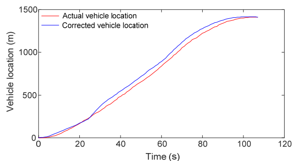
Fig. 17 Vehicle location after curve information correction
