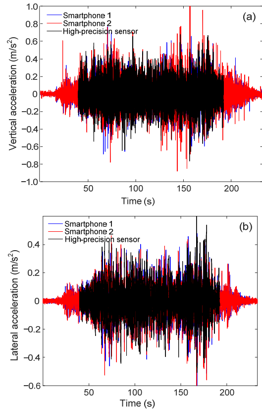
Fig. 11 Comparison of vertical (a) and lateral (b) accelerations obtained from smartphones and high-precision sensors
