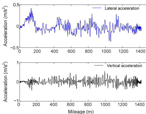
Fig. 18 Lateral and vertical accelerations of the vehicle in the spatial domain
