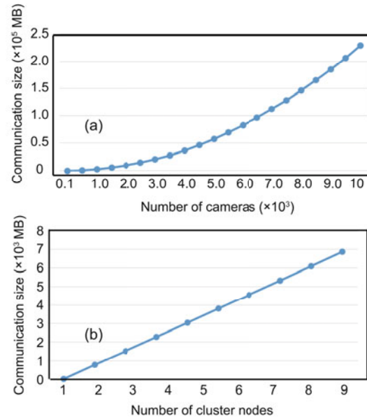
Fig. 5 Variation in the amount of traffic associated with the reduction of S : (a) r=4 and \text{cnp}=10 ; (b) m=1000 and \text{cnp}=10
