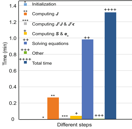
Fig. 2 Distribution of time consumption for each stage of sparse bundle adjustment
