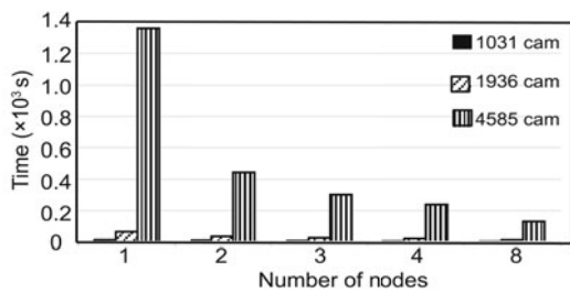
Fig. 11 Time consumption for solving the equation set
