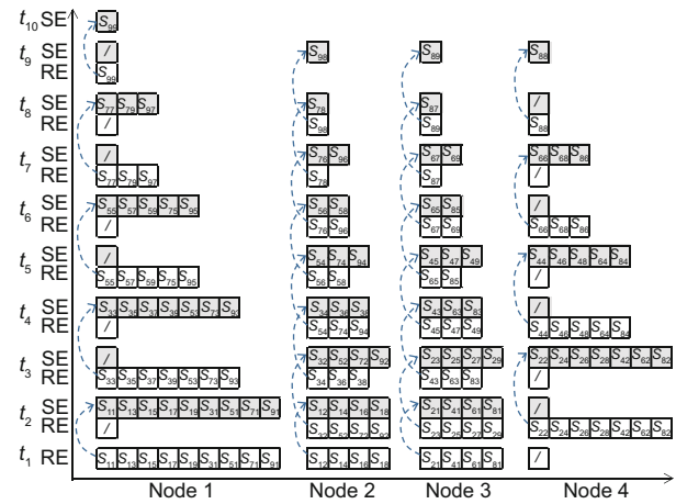
Fig. 9 Sequential chart showing how to solve the equation set based on asynchronous reduction
