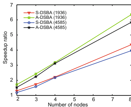
Fig. 14 Speedup ratio of DSBA
