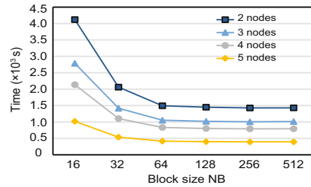
Fig. 12 Influence of block size on time consumption for solving the equation set
