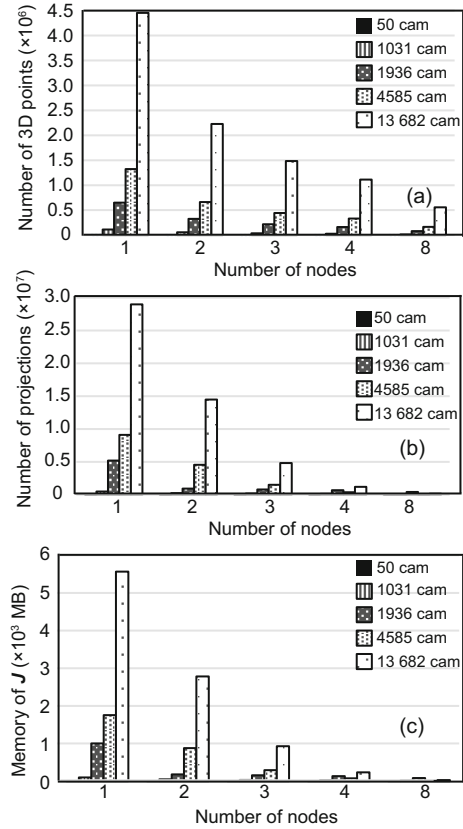
Fig. 10 Memory consumption of the DSBA algorithm: (a) variation in the number of 3D points; (b) variation in the number of projection points; (c) variation in the memory consumption of the Jacobian matrix
