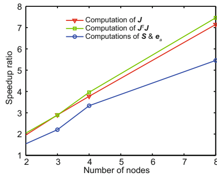
Fig. 13 Speedup ratio of the DSBA key steps
