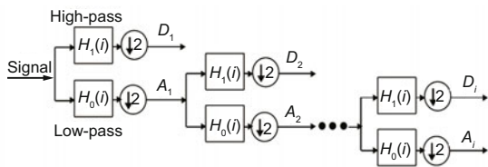
Fig. 4 Wavelet decomposition mechanism. High-pass: high-pass decomposition filter; low-pass: low-pass decomposition filter; \downarrow 2 : downsampling operation. A_1 , A_2 , and A_i are the approximation coefficients of the original signal at levels 1, 2, ..., i , respectively. D_1 , D_2 , and D_i are the detailed coefficients at levels 1, 2, ..., i , respectively
