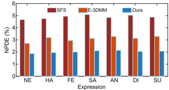
Fig. 10 Average normalized per-vertex depth errors (NPDEs) of the proposed and two counterpart methods for different expressions in the BU3DFE database. References to color refer to the online version of this figure
