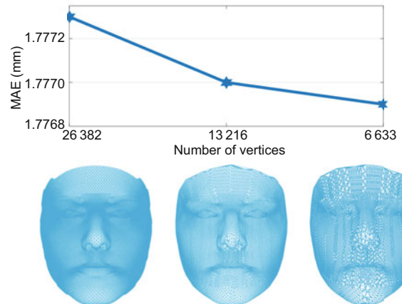
Fig. 9 MAEs of the proposed method over a fixed region of a 3D face when different numbers of vertices are used to represent that region
