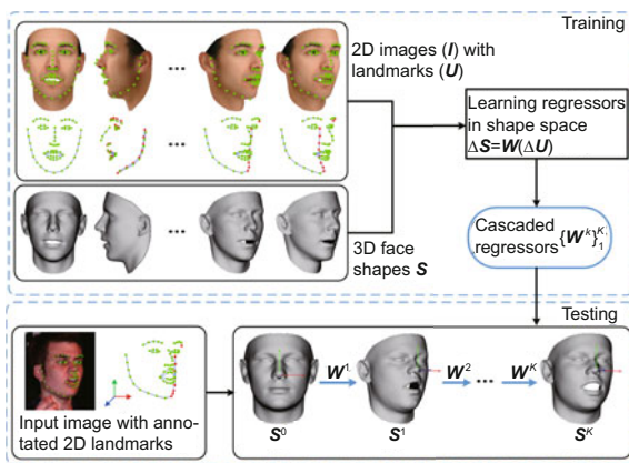
Fig. 3 Flowchart of the shape space cascaded regression based 3D face reconstruction method. Green and red points denote visible and invisible landmarks, respectively. Note that the method in this study does not require invisible landmarks’ locations as the input. References to color refer to the online version of this figure
