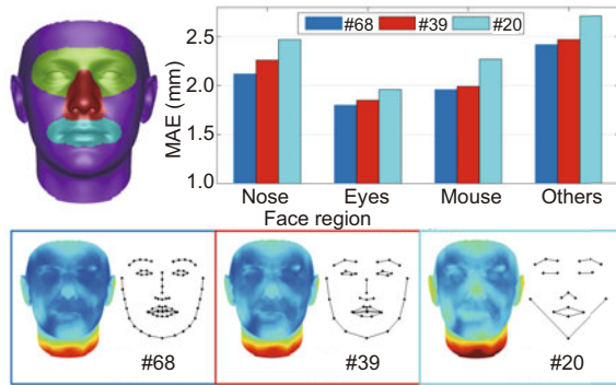
Fig. 7 MAEs of the proposed method in nose, eyes, mouse, and the other regions on the BFM test samples when different 2D landmarks are used. The bottom row shows the vertex-wise MAE maps, in which errors increase from blue to red. References to color refer to the online version of this figure
