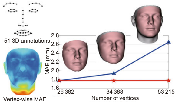
Fig. 8 MAEs of the proposed method over the whole set of 3D vertices (blue curve) and the subset of facial component vertices (red curve) on the BFM test samples as more vertices are included in the reconstructed 3D face shape and the 51 landmarks used remain unchanged. The vertex-wise MAE map shows the MAE per vertex in the 3D face (errors increase from blue to red). References to color refer to the online version of this figure
