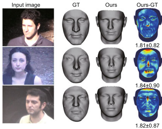
Fig. 12 Reconstruction results of the proposed method on three samples from the MICC database. From the first to the fourth columns: input images, ground-truth 3D shapes, reconstructed 3D shapes by the proposed method, and the corresponding MAE error maps, respectively
