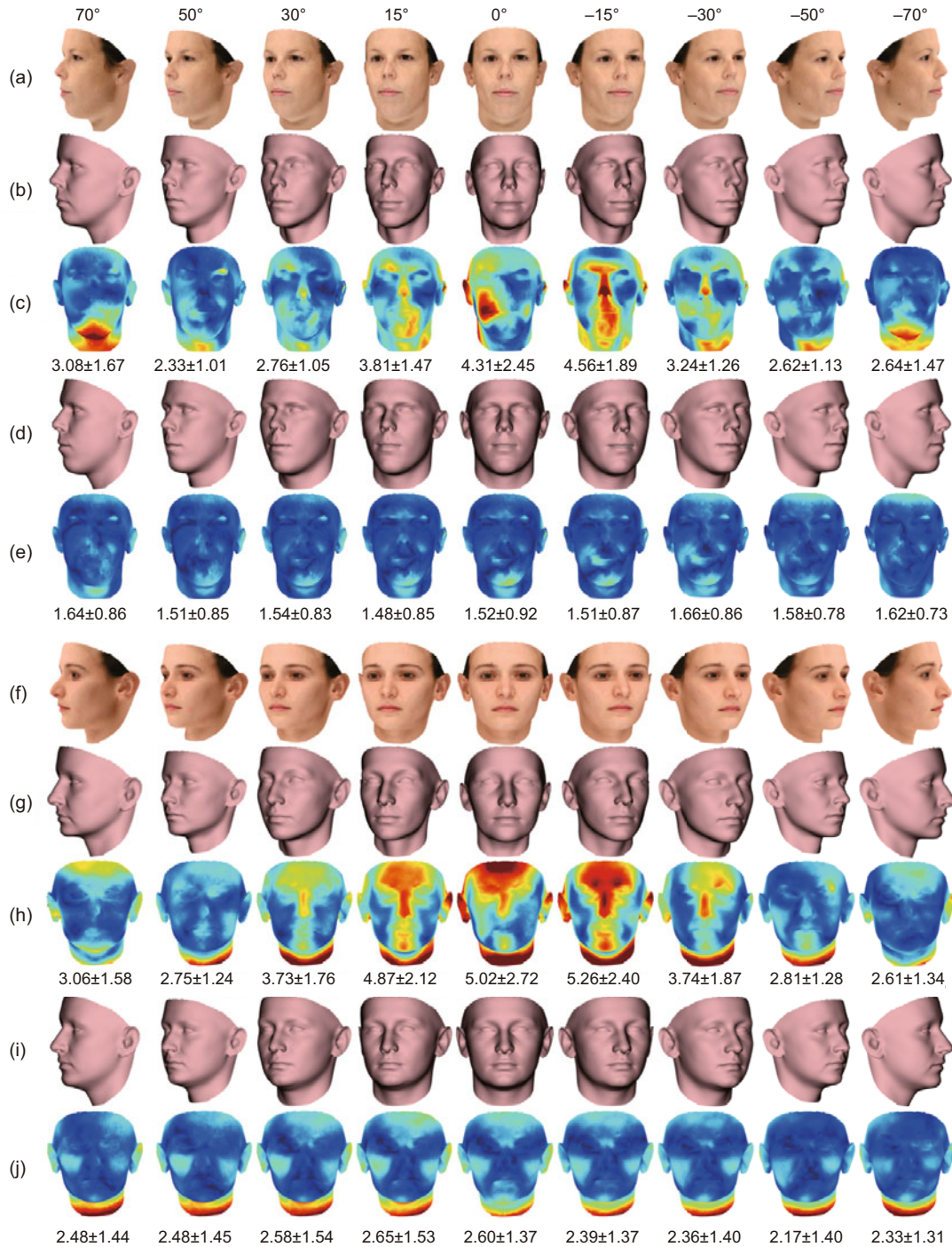
Fig. 6 Reconstruction results for two BFM samples at nine different poses: (a) and (f) are the input images; (b) and (g) are the reconstructed 3D face shapes by the SSF-3DMM method (Zhu et al. , 2014); (d) and (i) are those by the proposed method; (c) and (h) are the corresponding MAE error maps of the SSF-3DMM method; (e) and (j) are those by the proposed method. The colormap goes from dark blue to dark red (corresponding to an error from [0, 10]). The numbers under each of the error maps represent mean and standard deviation values (mm). References to color refer to the online version of this figure
