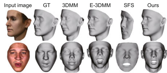
Fig. 2 Reconstruction results for images in the Basel face model (BFM) (top row) (Paysan et al., 2009) and BU3DFE (bottom row) (Yin et al., 2006) databases. From the left to the right columns: input images, ground-truth 3D shapes (GT), results by 3DMM (Bas et al., 2016), E-3DMM (Zhu XY et al., 2015), SFS (Kemelmacher-Shlizerman and Basri, 2011), and the proposed method
