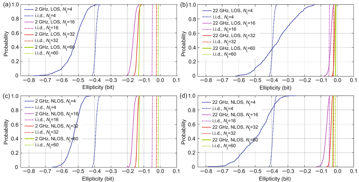
Fig. 10 Cumulative distribution functions of ellipticity for different numbers of Tx antennas with a 64-element planar array used at Tx: (a) at 2 GHz in the LOS scenario; (b) at 22 GHz in the LOS scenario; (c) at 2 GHz in the NLOS scenario; (d) at 22 GHz in the NLOS scenario (Tx: transmitter; RMS: root mean square; LOS: line-of-sight; NLOS: none-LOS)
