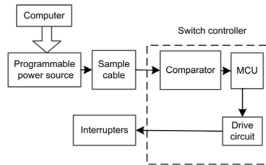
Fig. 3 Control logic of the proposed switching method
