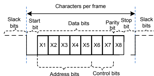
Fig. 5 Definition of the communication protocol
