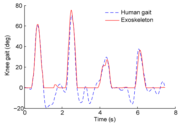
Fig. 10 Human gait trajectory in tracking the knee joint
