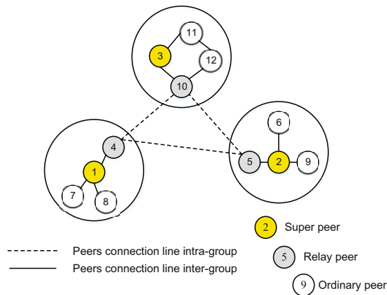
Fig. 1 An example of groups
