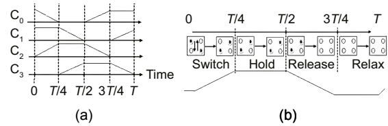
Fig. 6 Four-phase clocking (a) and QCA operation during one clock phase (b)
