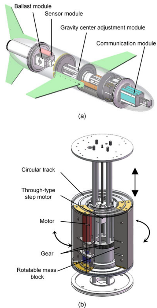
Fig. 3 Tiny underwater glider (a) and gravity center adjustment module (b)
