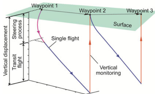
Fig. 1 Schedule diagram of lake monitoring pattern
