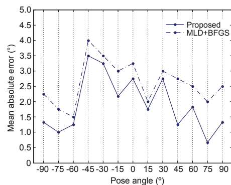
Fig. 11 Mean absolute errors of yaw angles achieved by the proposed and MLD+BFGS methods on the CMU Multi-PIE database
