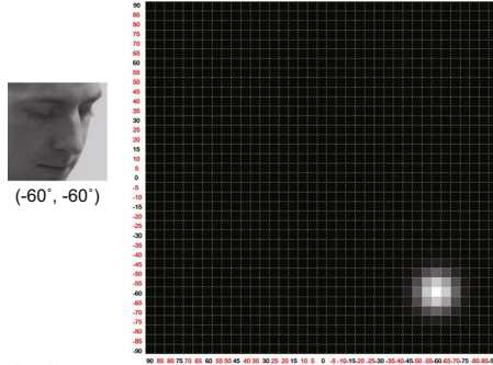
Fig. 2 A face image and its dense multivariate label distribution whose rows correspond to 37 possible pitch angles and columns to 37 possible yaw angles. The pose angles printed in red color are not included in the training data, i.e., the Pointing'04 database in this paper. References to color refer to the online version of this figure
