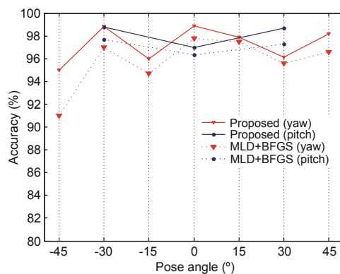
Fig. 10 Accuracies of yaw and pitch angles achieved by the proposed and MLD+BFGS methods on the CAS-PEAL database
