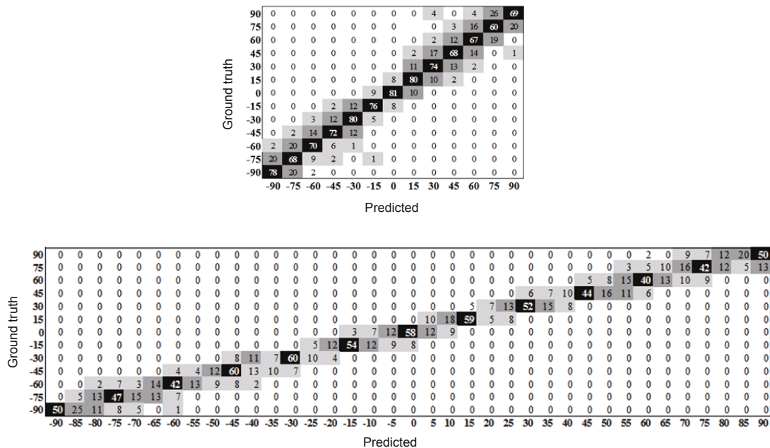
Fig. 9 Confusion matrices (in %) of the MLD+BFGS (up) and proposed (down) methods for yaw angles on the Pointing'04 database
