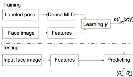
Fig. 3 Block diagram of the proposed dense multivariate label distribution (MLD) based head pose estimation method
