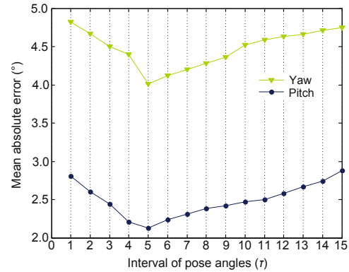
Fig. 7 Mean absolute error of yaw and pitch obtained using the proposed method with different \tau 's on the Pointing'04 database
