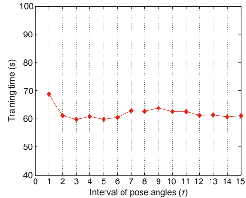
Fig. 8 Training time under different \tau for dense MLD on the Pointing'04 database
