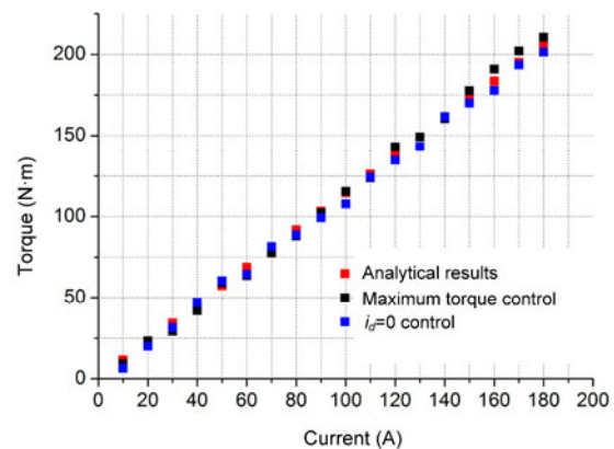
Fig. 19 PMSM torque output at different currents
