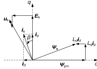
Fig. 5 Vector presentation of the PMSM
