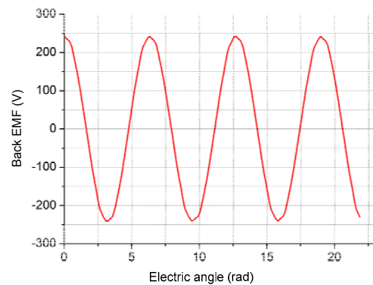
Fig. 18 Back EMF of PMSM
