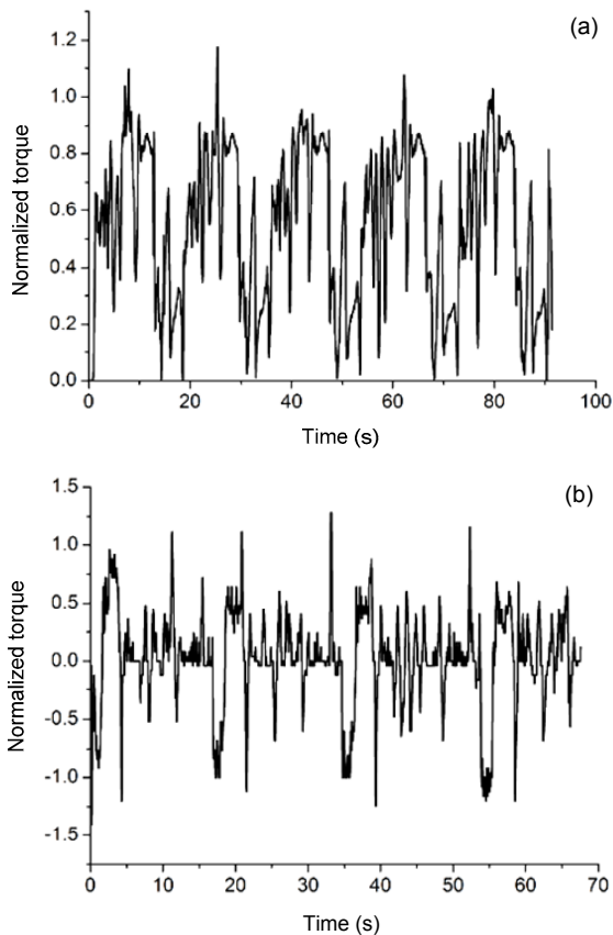
Fig. 2 Normalized mechanical torque (a) Hydraulic pump; (b) PMSM
