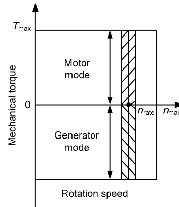
Fig. 3 PMSM mechanical characteristics
