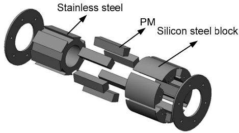
Fig. 4 Structure of the PMSM rotor
