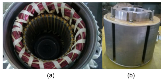
Fig. 16 Fabricated PMSM (a) Stator; (b) Rotor
