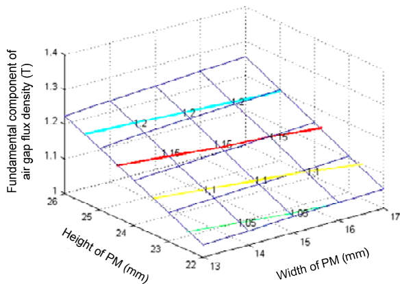
Fig. 10 Fundamental component of the air gap flux density varying with the PM dimension ( c_r=1 )
