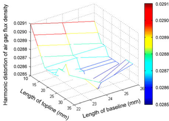
Fig. 13 Harmonic distortion of the air gap flux density varying with the PM dimension ( c_r=0.8 )
