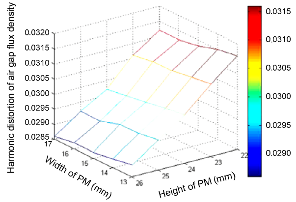
Fig. 11 Harmonic distortion of the air gap flux density varying with the PM dimension ( c_r=1 )
