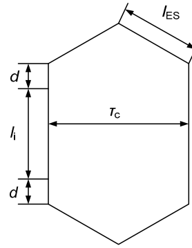
Fig. 7 Schematic diagram of a stator coil
