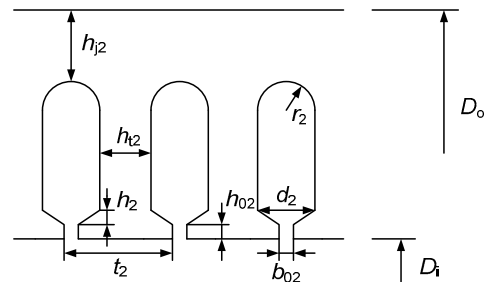
Fig. 6 Simplified cross section of the PMSM stator
