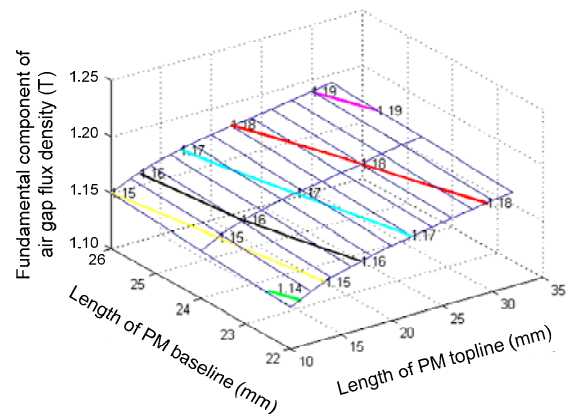
Fig. 12 Fundamental component of the air gap flux density varying with the PM dimension ( c_r=0.8 )
