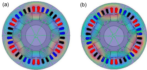
Fig. 15 Flux distribution without load (a) and at full load (b)
