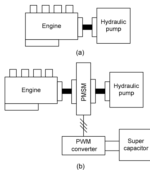
Fig. 1 Power transmission system (a) Traditional excavator; (b) Hybrid hydraulic excavator
