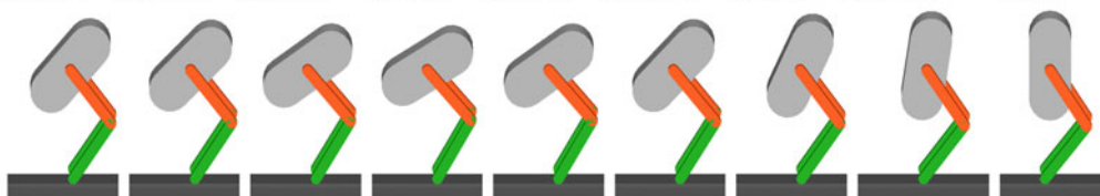
Fig. 9 Time-elapsd snapshots which show that the simulated biped recovers posture from 0.75 to 0 rad using ATB control (snapshots are sequenced from left to right at a 0.05 s interval)
