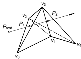
Fig. 7 Point-in-polyhedron test (PIPT)
