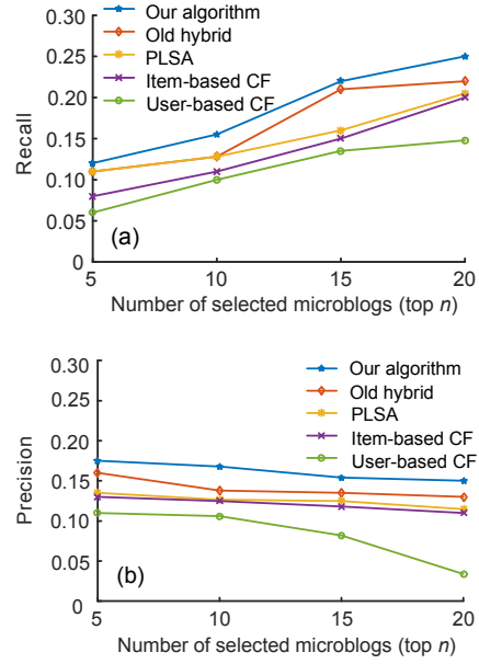
Fig. 5 Recalls (a) and precisions (b) with varying numbers of selected microblogs (top n ) under different algorithms
