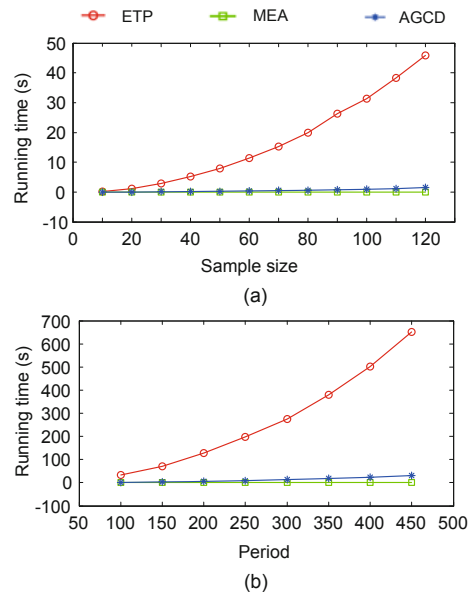
Fig. 6 Efficiency with regard to sample size N with p = 100 (a) and period p with N = 40 (b) ( r = 10, \lambda = 0.8 )
