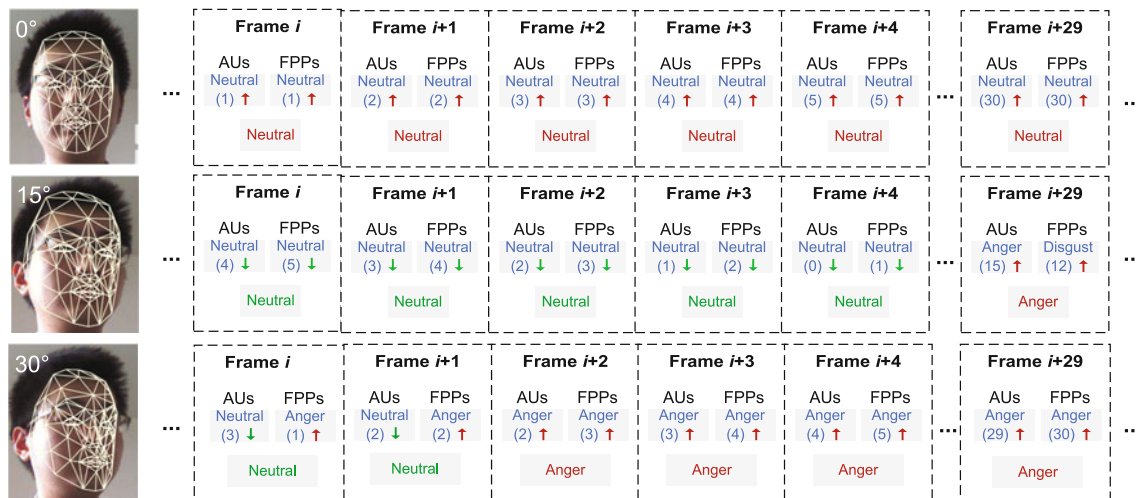
Fig. 15 Simplified operation examples on continuous 30 frames (frames i-(i+29) ). The first row is a sample for neutral emotion in the pose of 0°. The cumulative confidences of neutral keep rising in the AU and FPP channels, respectively. The second and third rows are samples for emotion changing from neutral to anger, where the cumulative confidence of neutral keeps dropping and confidence of anger keeps rising
