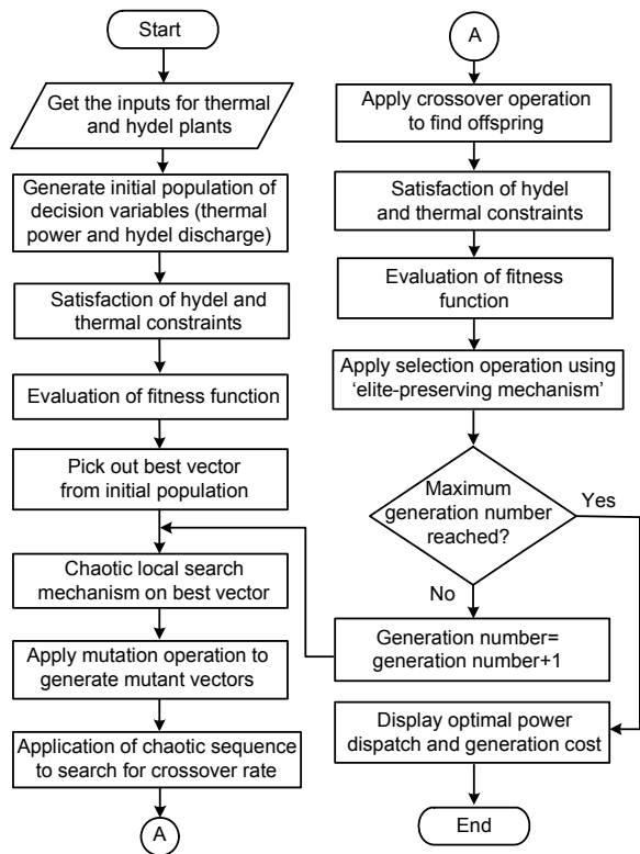
Fig. 1 Calculation chart of the proposed improved chaotic hybrid differential evolution algorithm
