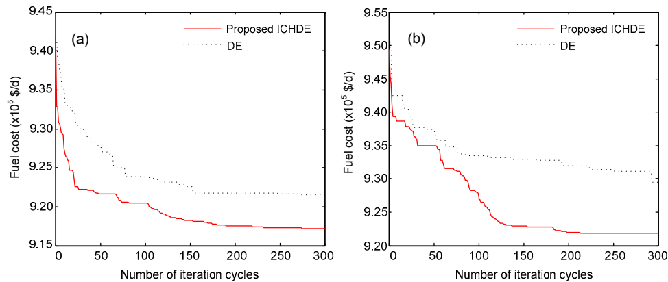
Fig. 3 Convergence characteristics of the differential evolution (DE) algorithm and the proposed improved chaotic hybrid differential evolution (ICHDE) algorithm: (a) case study 1; (b) case study 2
