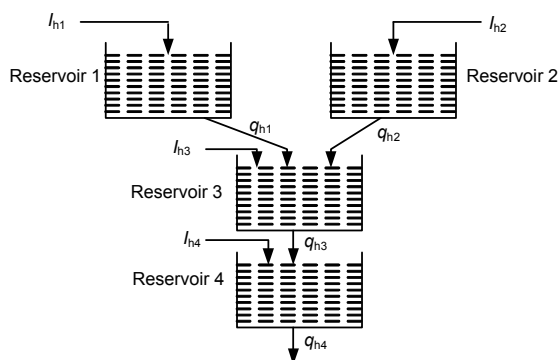
Fig. 2 Hydel network configuration
