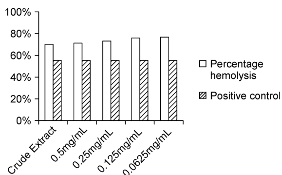
Figure 5 Anti-inflammatory activity of Streptomyces sp. VITPSA crude extract
