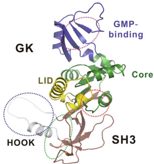
Figure 5 Possible protein–protein interaction sites in MAGUK SH3-GK tandems illustrated on the structure of the SAP97 SH3-GK supramodule. The GMP binding site colored deep purple; the potential ATP binding site colored red; the canonical SH3 binding pocket colored green; The HOOK region binding site colored blue.
