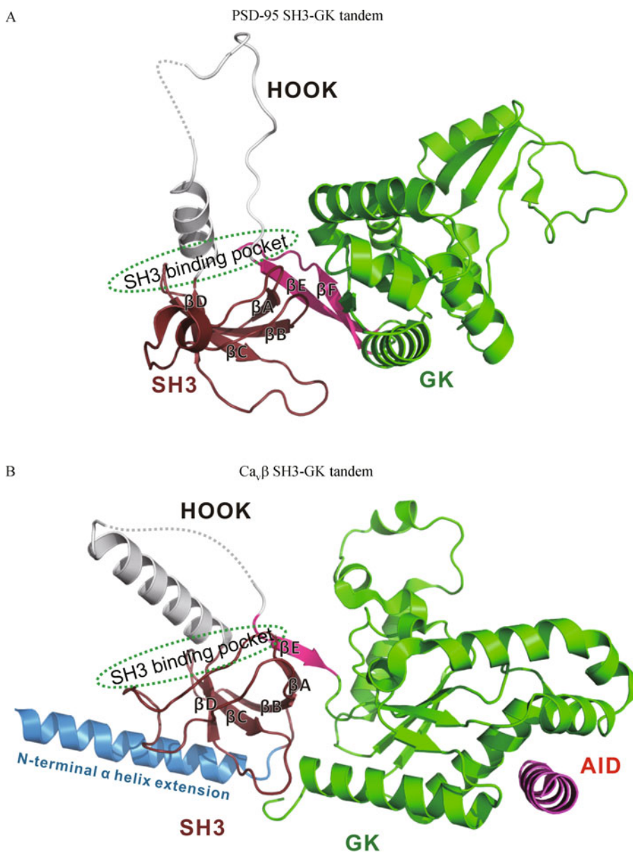
Figure 2 The SH3-GK supramodule. Ribbon diagrams of the PSD-95 SH3-GK tandem (PDB code: 1KJW) (A) and the \text{Ca}_v\beta SH3-GK tandem (PDB code: 1T3L) (B). The GK domain, the HOOK region and the split SH3 domain are colored green, gray and ruby-red, respectively. The coupling strands between SH3 and GK domain are colored magenta. The N-terminal helix extension in \text{Ca}_v\beta SH3-GK tandem is colored marine-blue.
