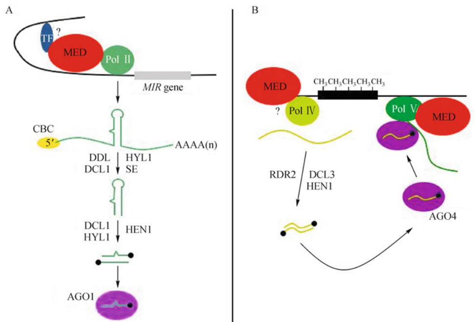
Figure 1 Roles of Mediator in noncoding RNA production in plants. (A) A diagram of the miRNA biogenesis pathway in Arabidopsis . Mediator recruits Pol II to promoters of microRNA genes to promote the transcription of MIR genes possibly by bridging the interaction between transcription factors and Pol II. A MIR gene is transcribed by Pol II into a capped and polyadenylated primary precursor, which undergoes processing to give rise to a small RNA duplex containing the miRNA and the antisense miRNA*. The duplex is methylated on the 2' OH of the 3' terminal nucleotides, and the miRNA strand is bound by AGO1, the miRNA effector protein. Known factors in miRNA biogenesis are indicated. TF, transcription factor; CBC, cap binding complex; DDL, DAWDLE; DCL1, DICER-LIKE1; HYL1, HYPOPLASTIC LEAVES1; SE, SERRATE; HEN1, HUA ENHANCER1; AGO1, ARGONAUTE1. (B) A diagram of siRNA biogenesis and siRNA-mediated transcriptional gene silencing at repeats and transposable elements. The black rectangle represents a repeats- or transposable element-containing locus that harbors DNA methylation (CH 3 ). Pol IV presumably transcribes the locus into a single-stranded noncoding RNA, which eventually gives rise to 24 nt siRNAs through the activities of RNA-dependent RNA polymerase 2 (RDR2), DICER-LIKE3 (DCL3), and HEN1. The siRNAs are bound by AGO4, a major siRNA effector protein. The AGO4/siRNA complexes are thought to be recruited back to homologous chromatin by noncoding scaffold transcripts produced by Pol V, and at some loci, Pol II. It is not known whether Mediator assists Pol V in the production of noncoding RNAs, but it is required for noncoding RNA production by Pol II. The small black dots in (A) and (B) indicate the methyl group on the 3' terminal ribose of small RNAs.
