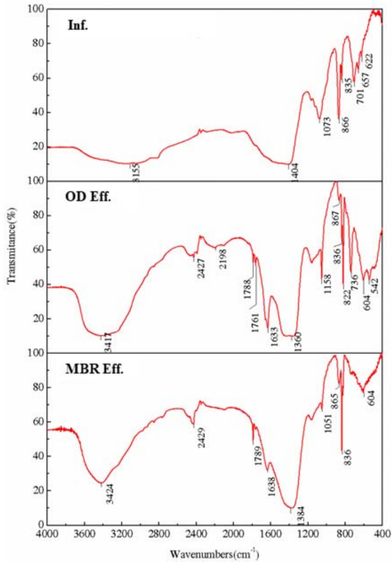
Fig. S1 FTIR results of influent and effluent of OD and MBR, where MBR effluent showed fewer characteristic peaks than OD
