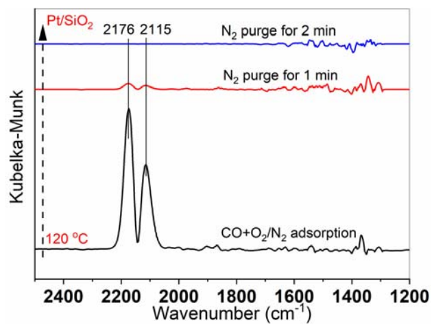
Fig. S2 In situ FTIR spectra of CO adsorbed at 120°C followed by N 2 purging on Pt/SiO 2 catalysts
