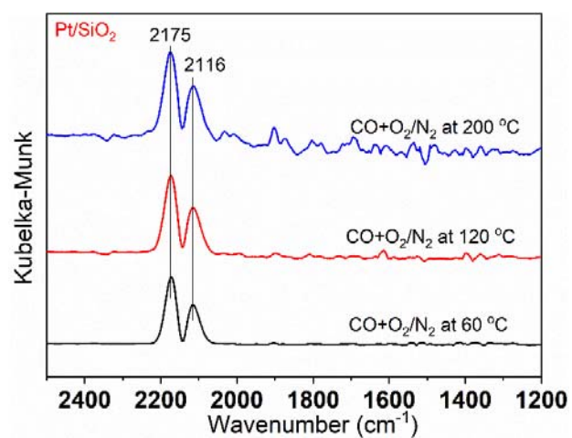
Fig. S3 In situ FTIR spectra of CO and O 2 co-adsorption at 60°C, 120°C, and 200°C on Pt/SiO 2 catalysts
