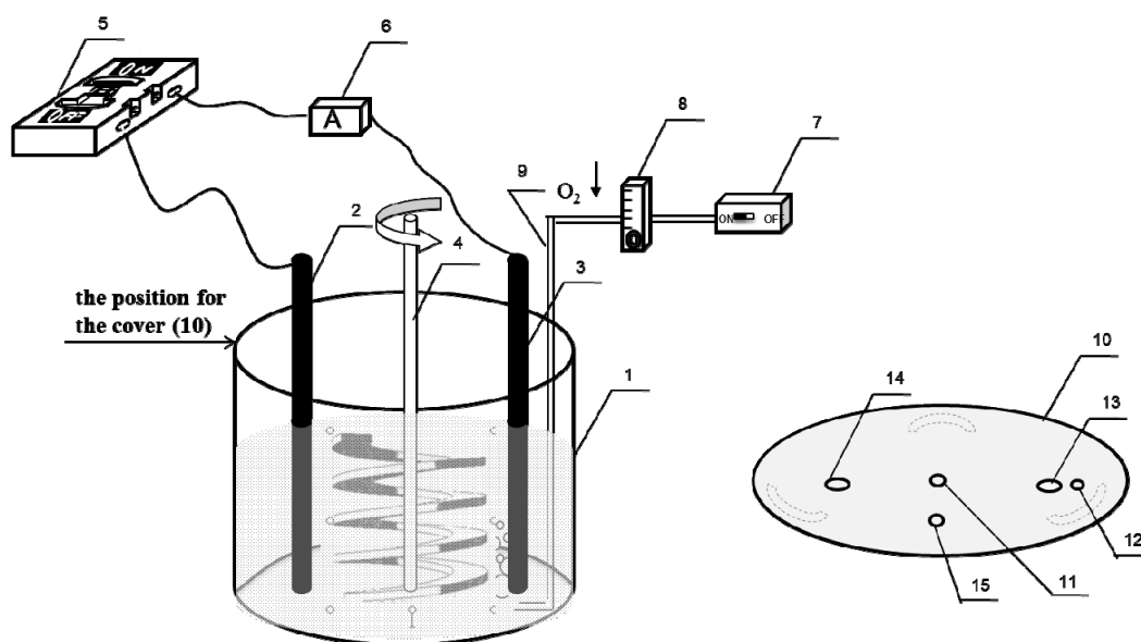
1. glass cylindrical vessel 2. iron anode 3. graphite cathode 4. stirrer 5. direct power supply 6. amperemeter 7. pump 8. gas flow meter 9. aeration pipe 10. adjustable fitted cover 11. hole of stirrer 12. hole of aeration 13. hole of cathode 14. hole of anode 15. hole of sampling
