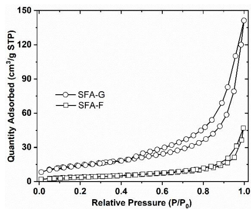
Fig. S1 Nitrogen adsorption-desorption isotherms of SFA-G and SFA-F.
