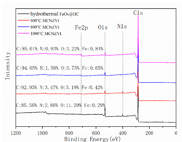
Figure S1. XPS Full spectrum analysis of hydrothermal FeOx@HC, Fe@HC obtained by calcining at different temperatures
