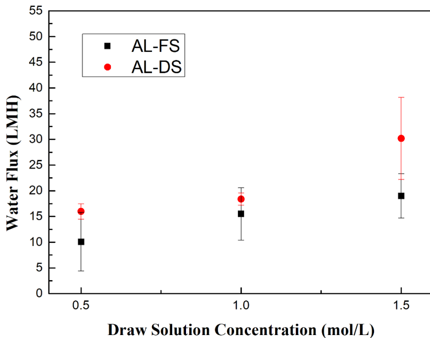
Fig. S1 The dependence of the water flux of TFC-D-1 on the concentration of DS ranging from 0.5 mol/L to 1.5 mol/L NaCl solution, where DI water was used as FS. The error bars were calculated based on three independently repeated tests.
