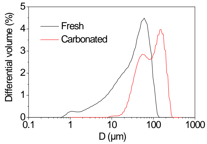
Fig. S1 Particle size distribution of fresh and carbonated carbide slag.
