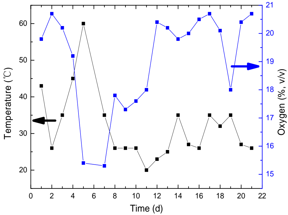
Fig. A1 The evolution of temperature and volumetric oxygen content during sludge stabilization
