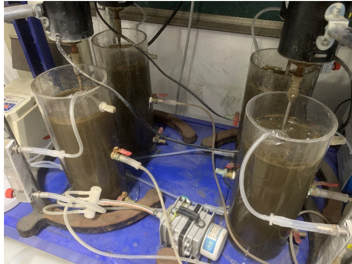
Fig. S1 Laboratory setup of sequencing batch reactors.
