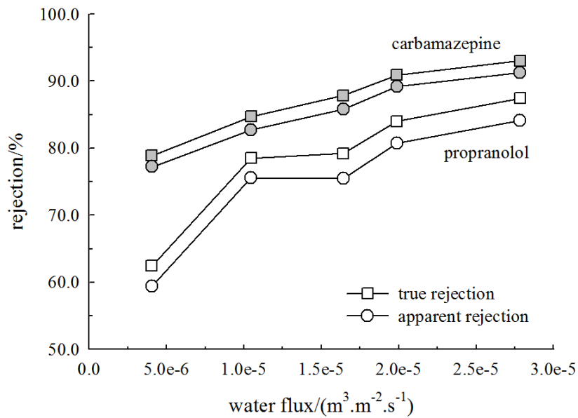
Fig. A2 Effect of concentration polarization on rejection of propranolol and carbamazepine by the NF270 membrane
