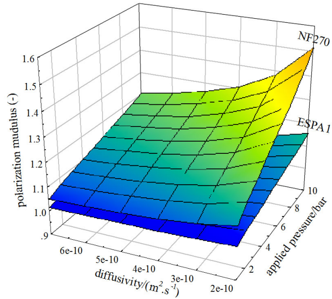
Fig. A1 Dependence of the concentration polarization modulus on the applied pressure and the solute diffusivity for the NF270 and ESPA1 membranes
