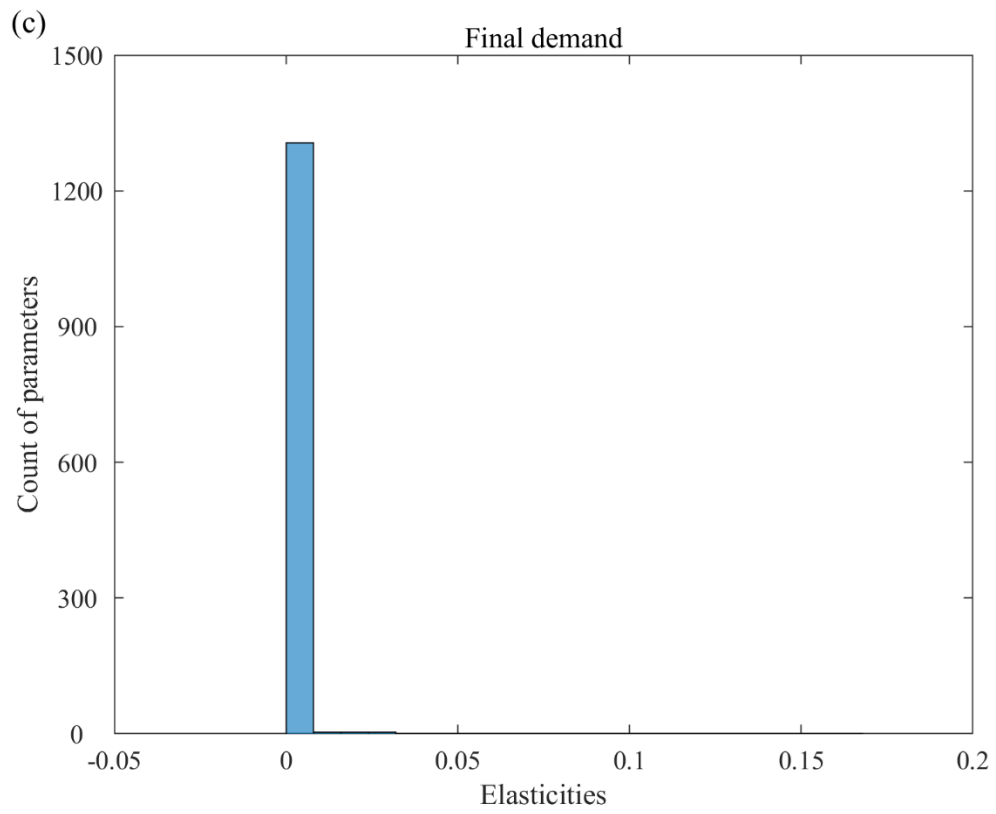
Fig. S1. Distributions of the elasticities for global GHG emissions driven by food consumption in China.
