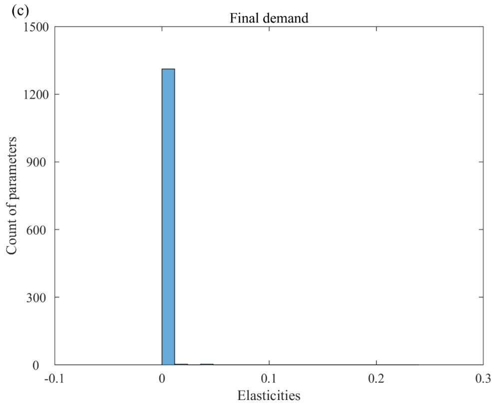
Fig. S2. Distributions of the elasticities for global P emissions driven by food consumption in China.
