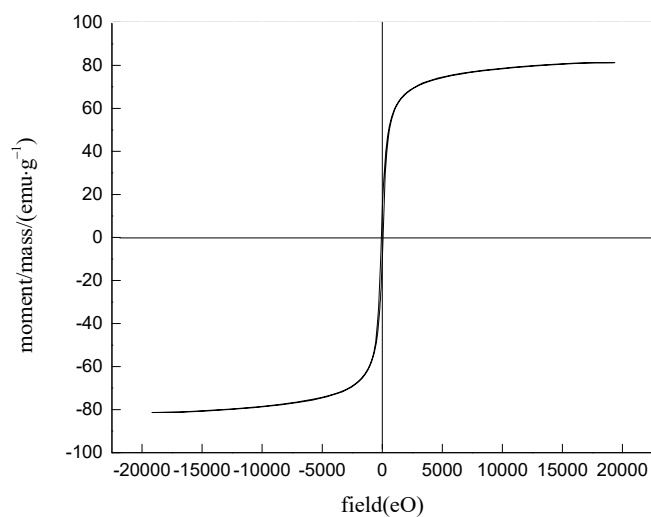
Fig. S1 VSM curve of the \text{Fe}_3\text{O}_4 nanoparticles from simulated wastewater with the combination of three promoters
