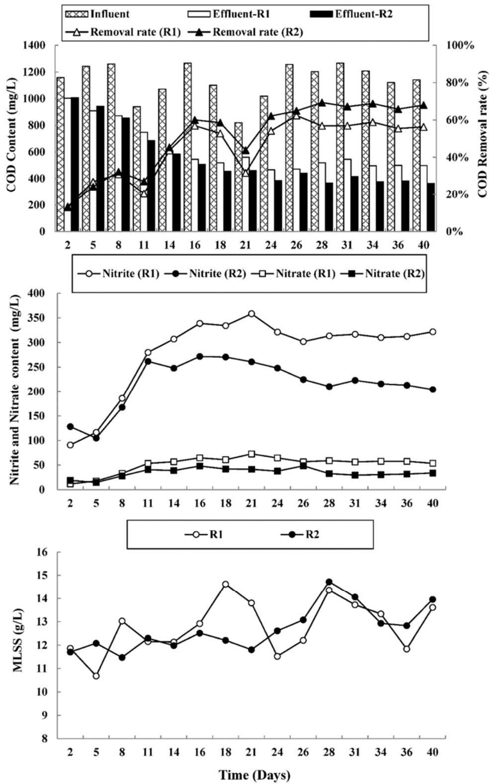
Fig. A1 The change of original COD, nitrite, nitrate and MLSS during 40 days
