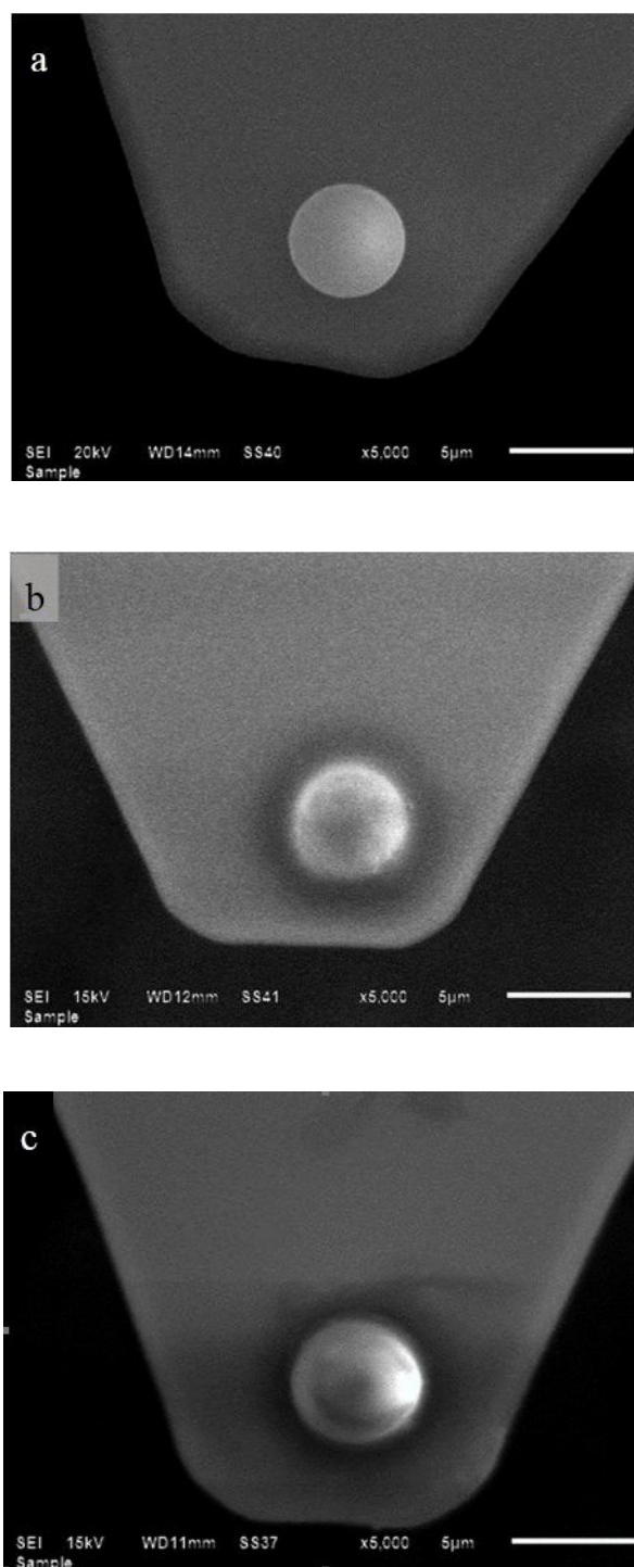
Fig. S1 SEM images of modified AFM colloidal probes: (a) the SiO 2 colloidal probe; (b) the PVDF/PVA membrane-coated colloidal probe; and (c) the BSA-coated colloidal probe
